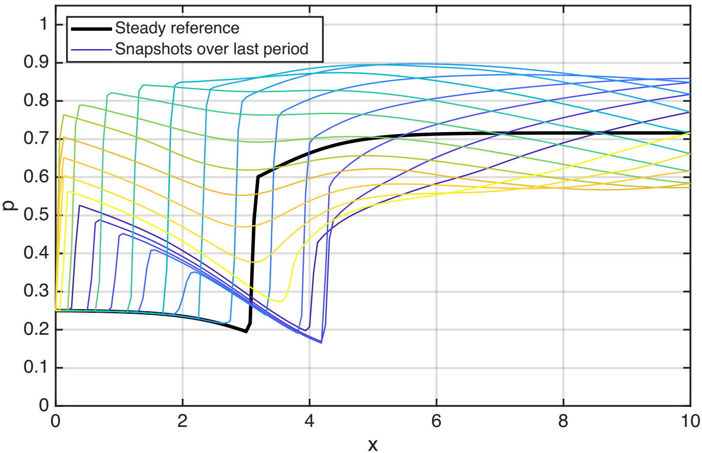
Unsteady pressure envelope (last period): \Delta p_{\text{var}}=0.20 , T=1.00
