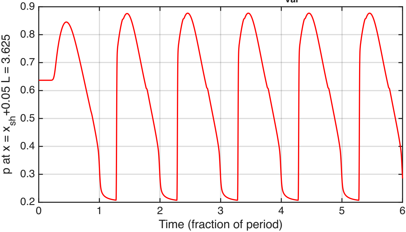
Probe pressure history (6 periods): \Delta p_{\text{var}}=0.20 , T=1.00
