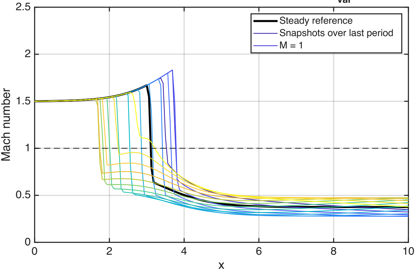
Unsteady Mach-number envelope (moderate case: \Delta p_{\text{var}}=0.10 , T=1 )
