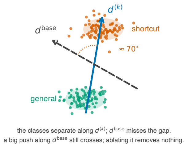
(b) Why the dissociation happens
