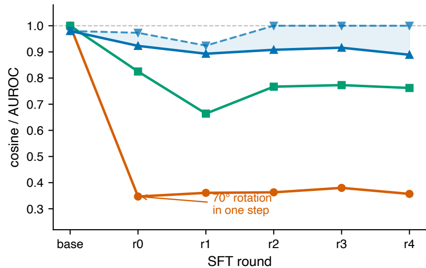
(a) Direction rotates; fresh probe recovers, frozen does not
