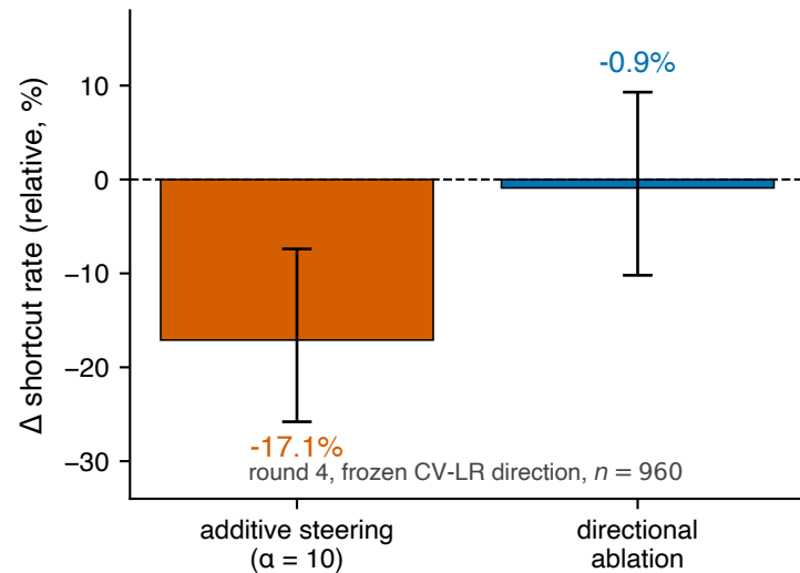
(c) Same direction. Opposite verdicts.
