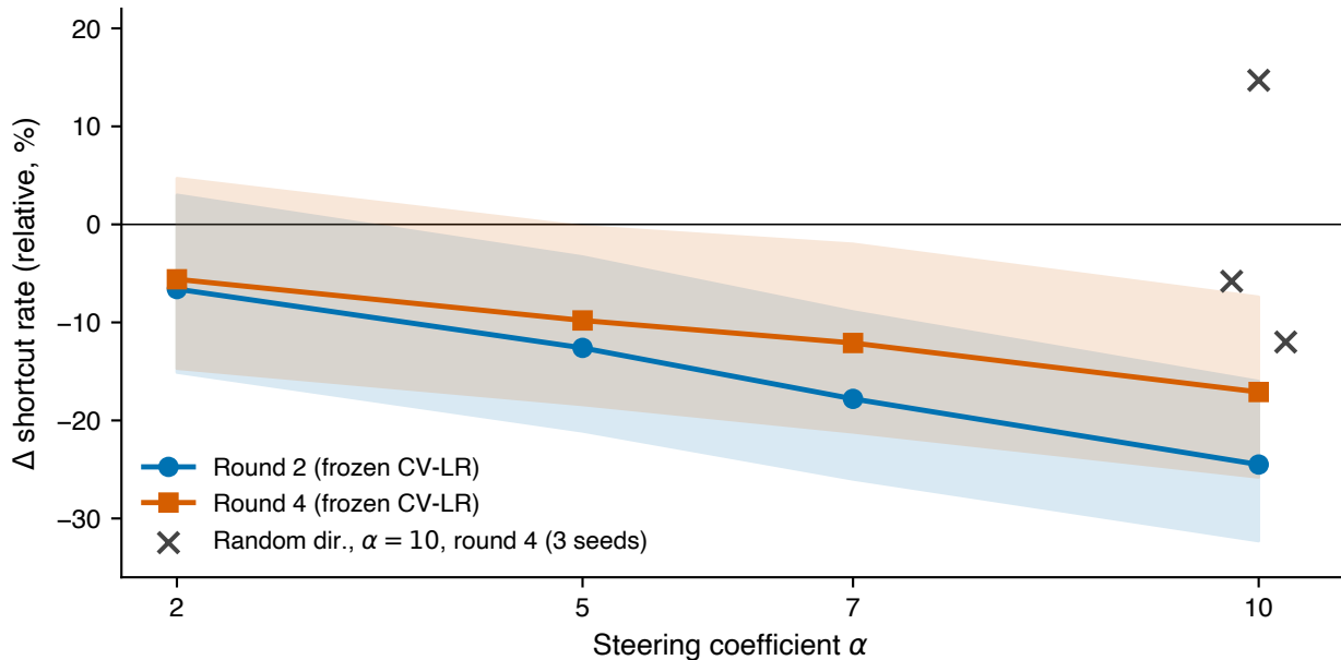
Additive steering: monotonic dose-response at both checkpoints
