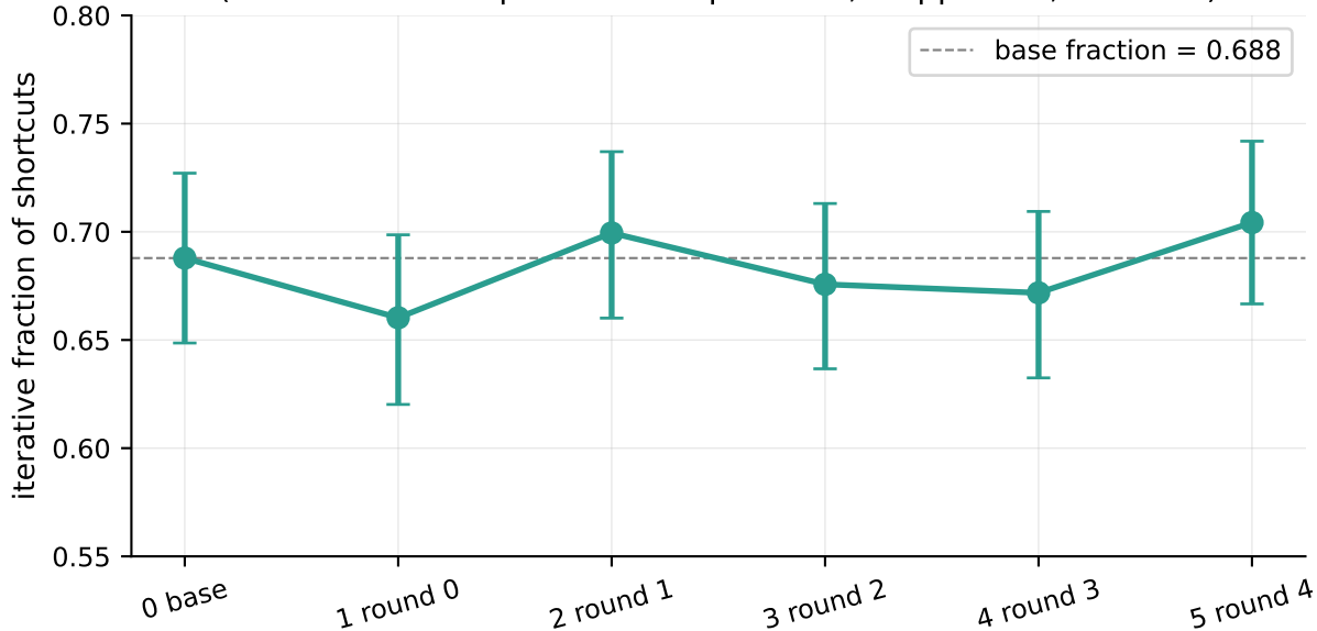
Shortcut strategy distribution is stable across training (base vs round 4 permutation p = 0.57 ; \pm 4pp band, no trend)
