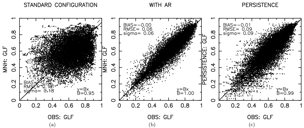
Figure 28: ground layer fraction (no unit): (a) STANDARD CONFIGURATION, (b) WITH AR (1H), (c) PERSISTENCE (1H)
