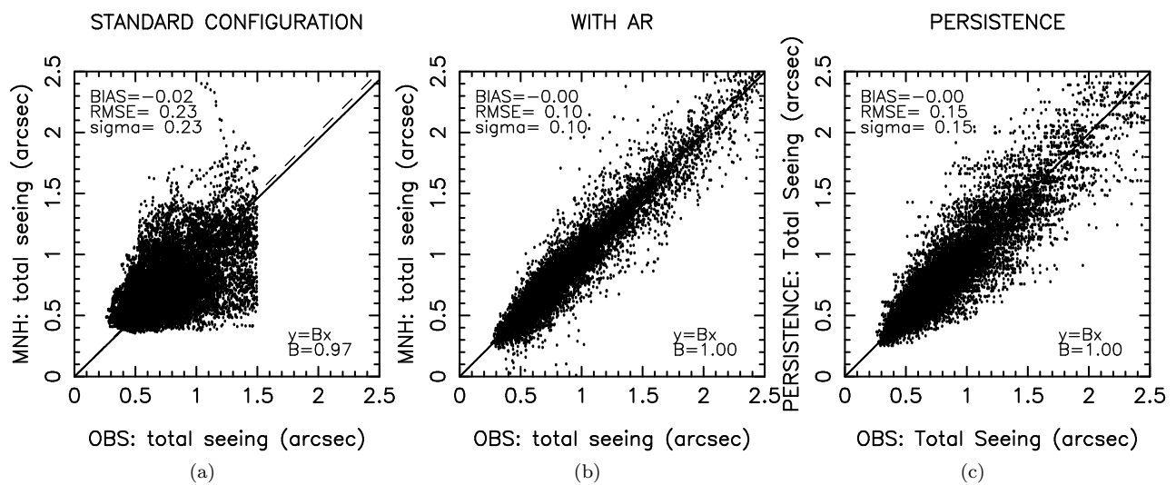
Figure 40: total seeing (arcsec): (a) STANDARD CONFIGURATION ( < 1.5'' ), (b) WITH AR (1H), (c) PERSISTENCE (1H).
