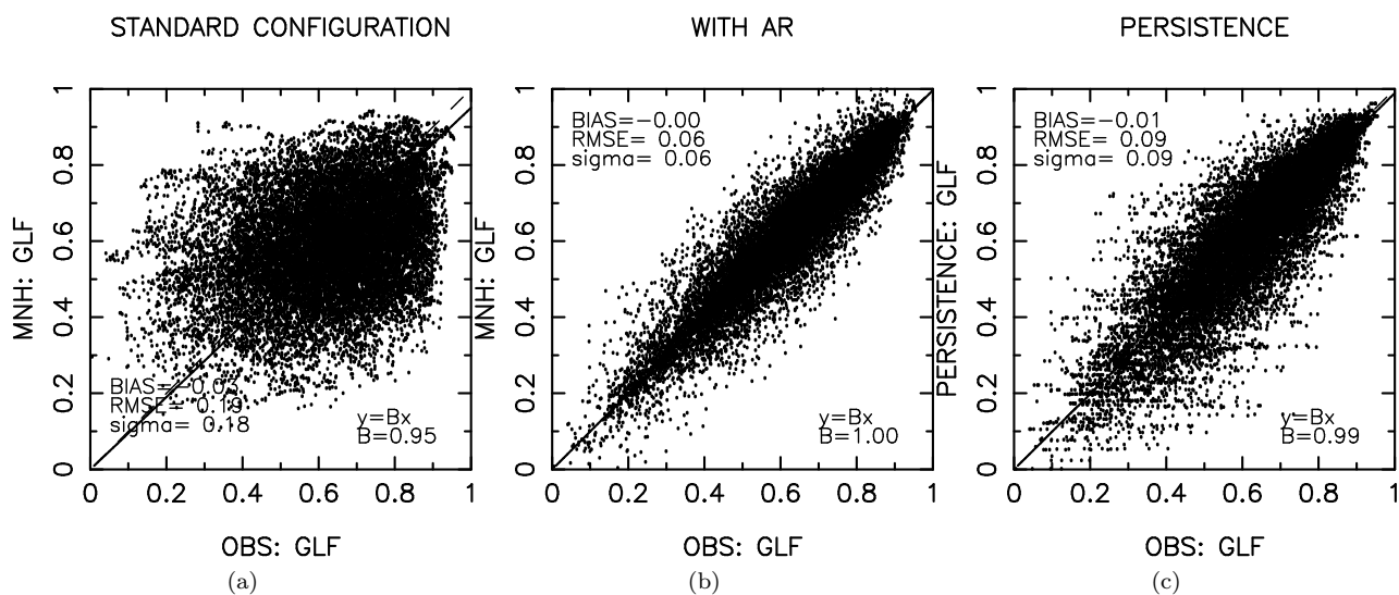
Figure 35: ground layer fraction (no unit): (a) STANDARD CONFIGURATION, (b) WITH AR (1H), (c) PERSISTENCE (1H)
