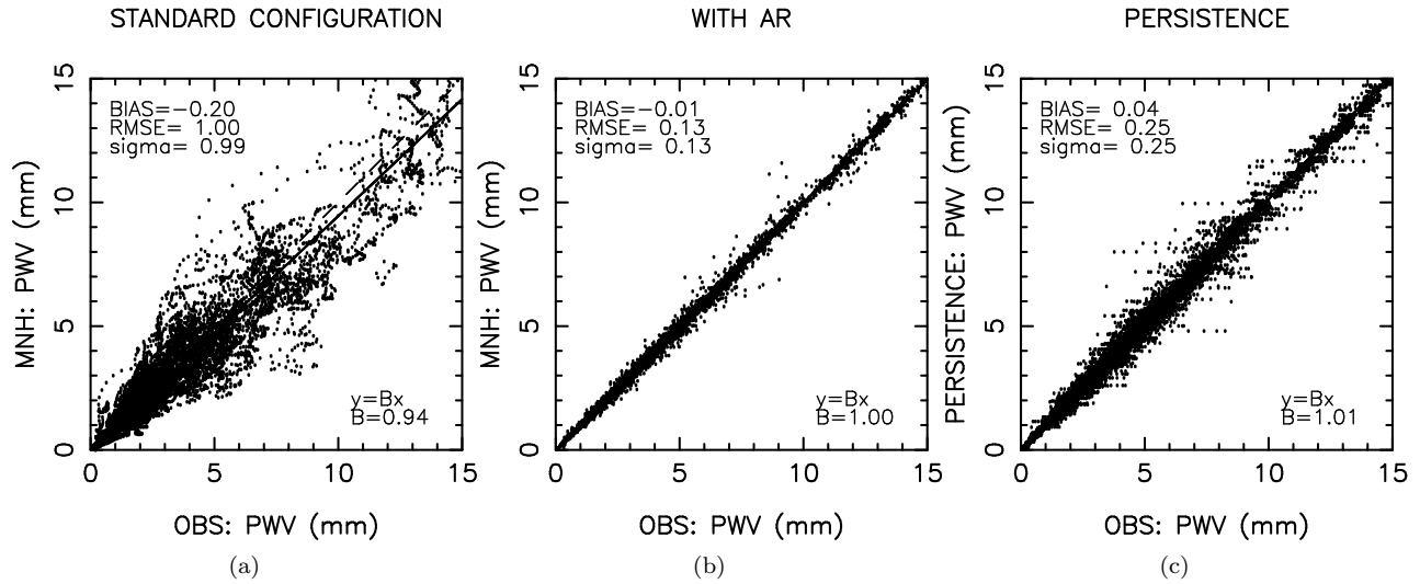
Figure 39: precipitable water vapor (mm): (a) STANDARD CONFIGURATION, (b) WITH AR (1H), (c) PERSISTENCE (1H).
