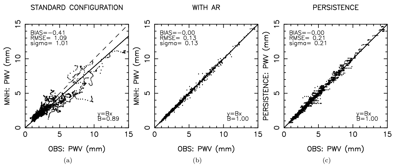
Figure 11: precipitable water vapor (mm): (a) STANDARD CONFIGURATION, (b) WITH AR (1H), (c) PERSISTENCE (1H).
