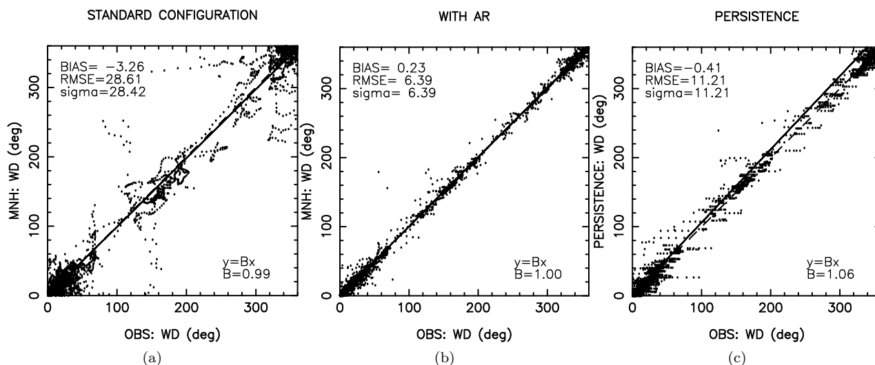
Figure 2: wind direction (degree): (a) STANDARD CONFIGURATION, (b) WITH AR (1H), (c) PERSISTENCE (1H).
