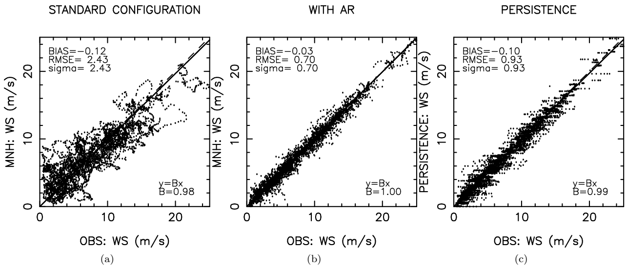
Figure 1: wind speed ( ms^{-1} ): (a) STANDARD CONFIGURATION, (b) WITH AR (1H), (c) PERSISTENCE (1H) for night1.
