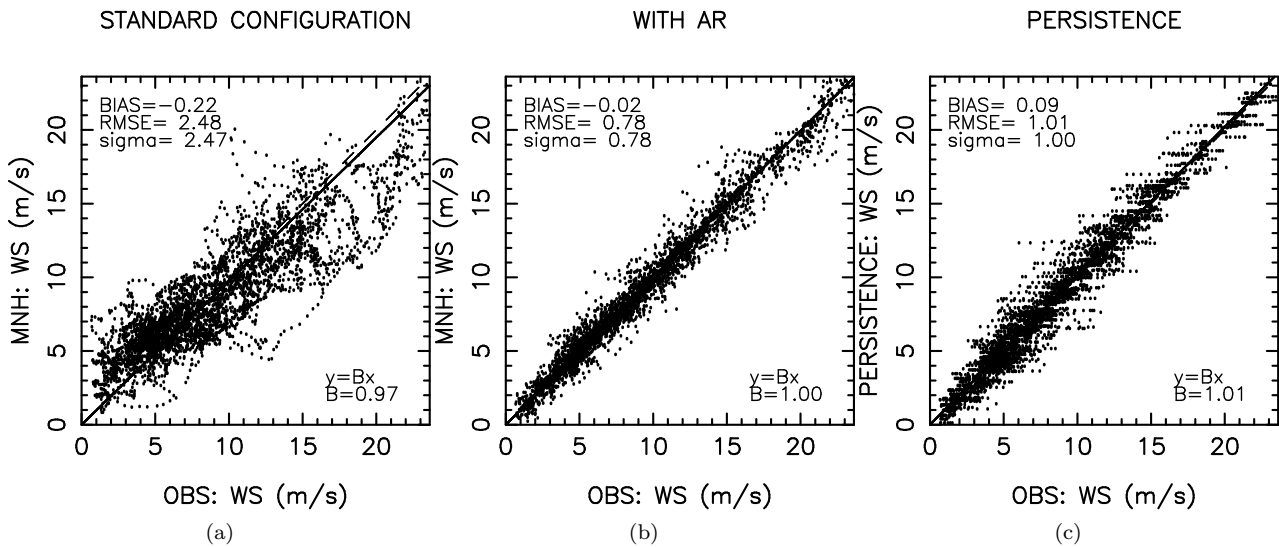
Figure 8: wind speed ( ms^{-1} ): (a) STANDARD CONFIGURATION, (b) WITH AR (1H), (c) PERSISTENCE (1H) for day1.
