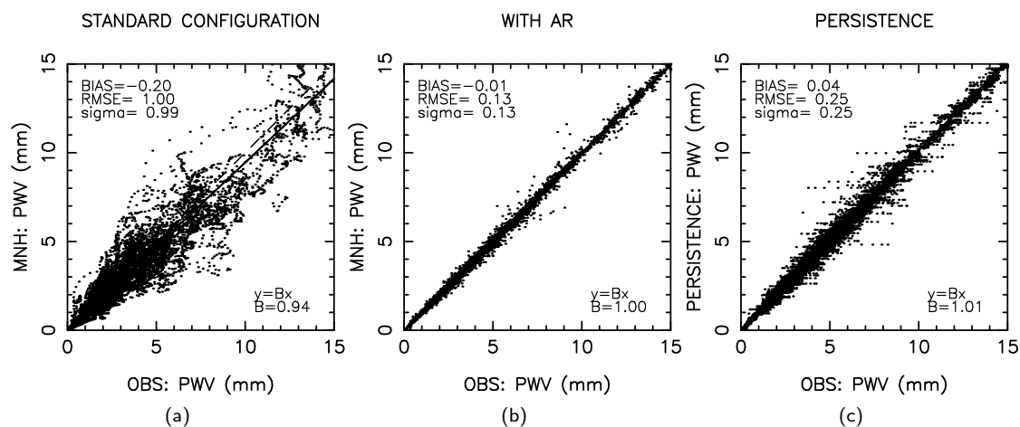
Figure 4: precipitable water vapor (mm): (a) STANDARD CONFIGURATION, (b) WITH AR (1H), (c) PERSISTENCE.
