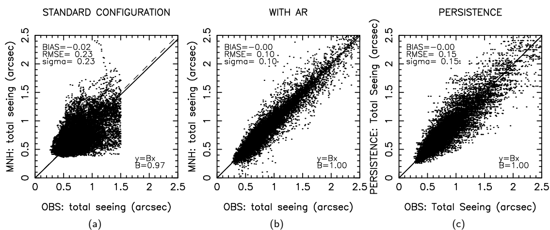
Figure 5: total seeing (arcsec): (a) STANDARD CONFIGURATION ( < 1.5'' ), (b) WITH AR (1H), (c) PERSISTENCE.
