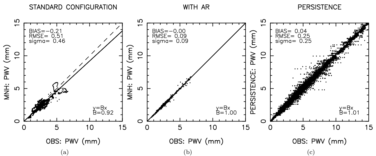
Figure 16: precipitable water vapor (mm): (a) STANDARD CONFIGURATION, (b) WITH AR (1H), (c) PERSISTENCE (1H).
