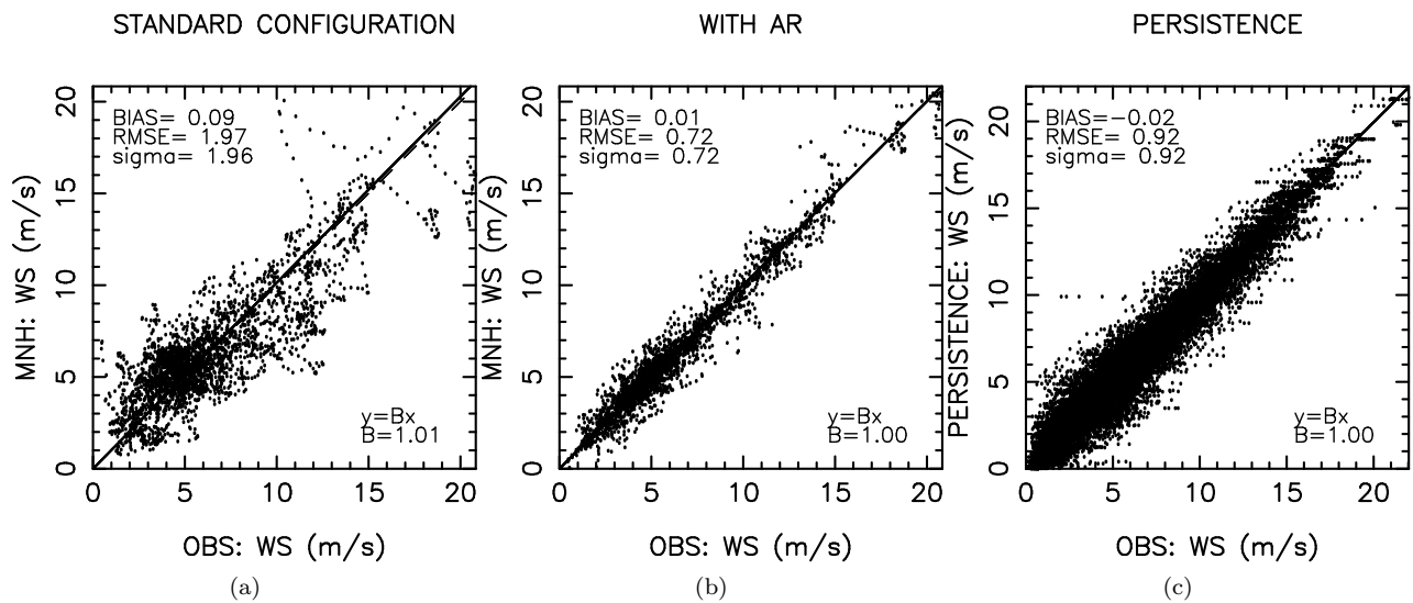
Figure 21: wind speed ( m s^{-1} ): (a) STANDARD CONFIGURATION, (b) WITH AR (1H), (c) PERSISTENCE (1H).
