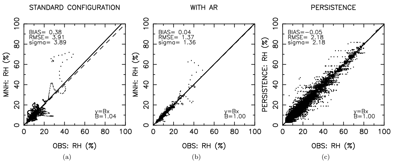
Figure 15: relative humidity (percent): (a) STANDARD CONFIGURATION, (b) WITH AR (1H), (c) PERSISTENCE (1H).
