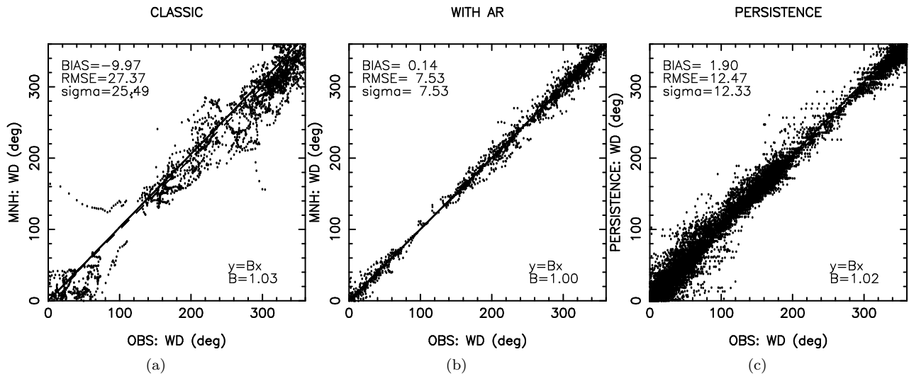
Figure 14: wind direction (degree): (a) STANDARD CONFIGURATION, (b) WITH AR (1H), (c) PERSISTENCE (1H).
