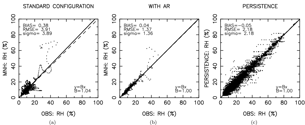
Figure 11: relative humidity (percent): (a) STANDARD CONFIGURATION, (b) WITH AR (1H), (c) PERSISTENCE (1H).
