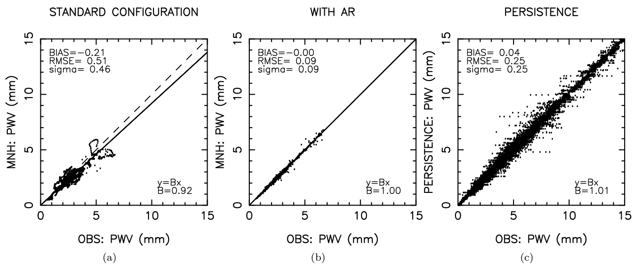
Figure 8: precipitable water vapor (mm): (a) STANDARD CONFIGURATION, (b) WITH AR (1H), (c) PERSISTENCE (1H).
