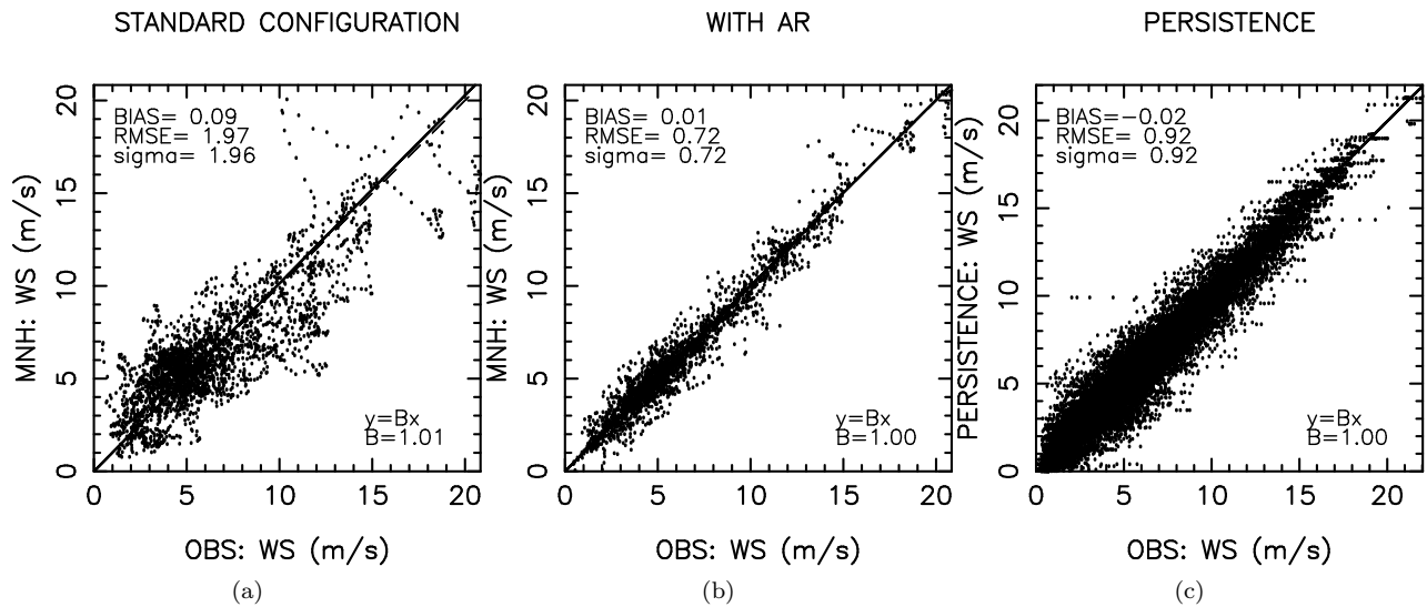
Figure 5: wind speed ( ms^{-1} ): (a) STANDARD CONFIGURATION, (b) WITH AR (1H), (c) PERSISTENCE (1H).
