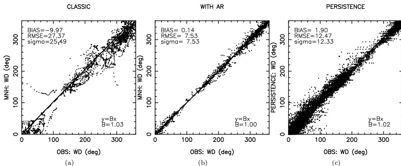
Figure 18: wind direction (degree): (a) STANDARD CONFIGURATION, (b) WITH AR (1H), (c) PERSISTENCE (1H).
