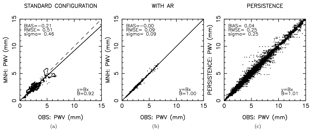
Figure 12: precipitable water vapor (mm): (a) STANDARD CONFIGURATION, (b) WITH AR (1H), (c) PERSISTENCE (1H).
