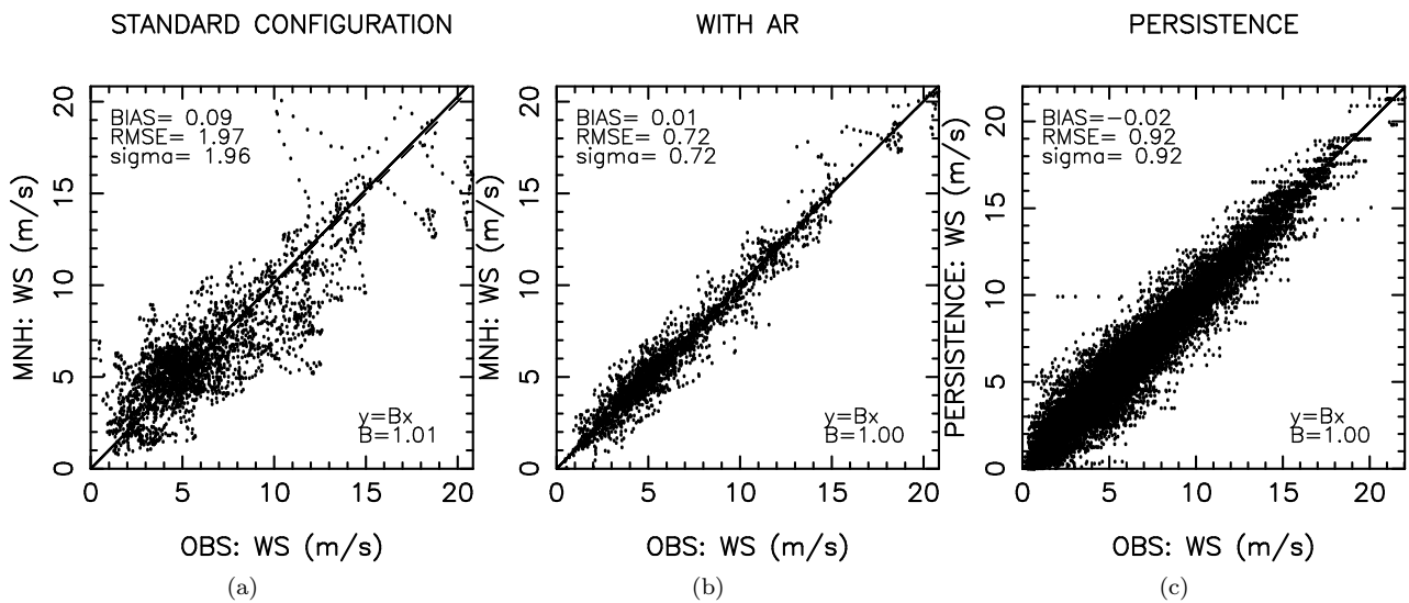
Figure 17: wind speed ( ms^{-1} ): (a) STANDARD CONFIGURATION, (b) WITH AR (1H), (c) PERSISTENCE (1H).
