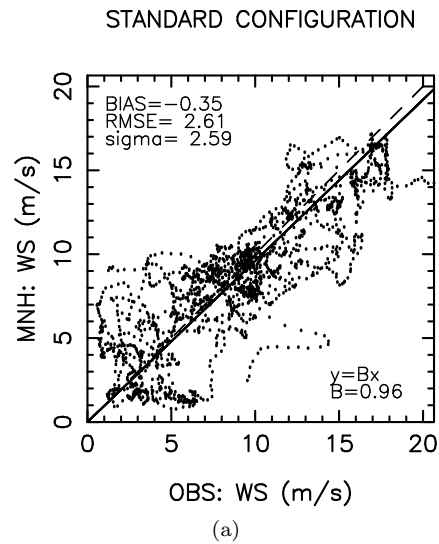
Figure 23: night3 - wind speed ( ms^{-1} ): STANDARD CONFIGURATION
