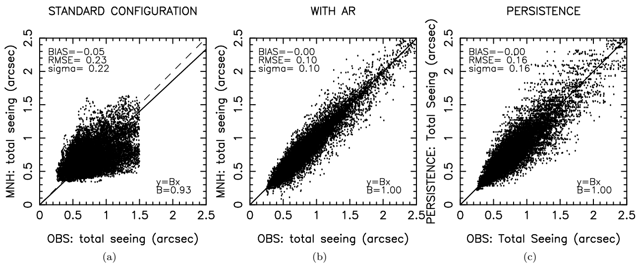
Figure 4: night1 - total seeing (arcsec): (a) STANDARD CONFIGURATION (< 1.5"), (b) WITH AR (1H), (c) PERSISTENCE (1H)
