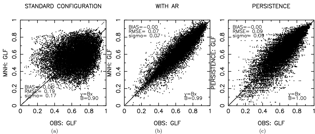
Figure 6: night1 - ground layer fraction (dimensionless): (a) STANDARD CONFIGURATION, (b) WITH AR (1H), (c) PERSISTENCE (1H)
