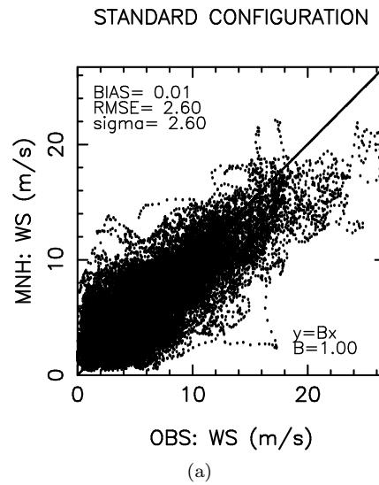
Figure 10: night2 - wind speed ( ms^{-1} ): STANDARD CONFIGURATION
