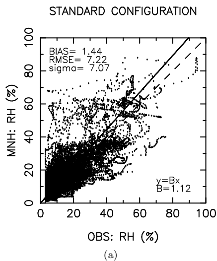
Figure 12: night2 - relative humidity (percent): STANDARD CONFIGURATION
