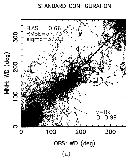
Figure 22: night3 - wind direction (degree): STANDARD CONFIGURATION
