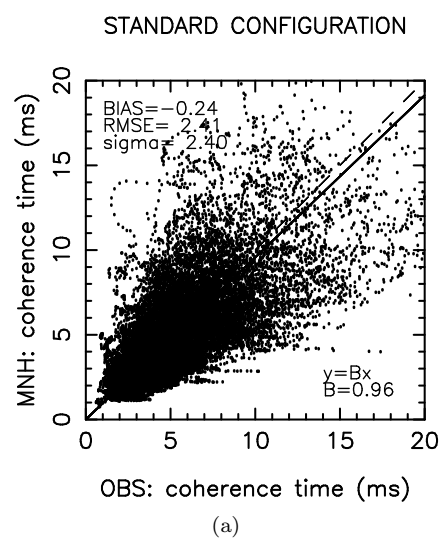
Figure 15: night2 - wavefront coherence time (ms): STANDARD CONFIGURATION
