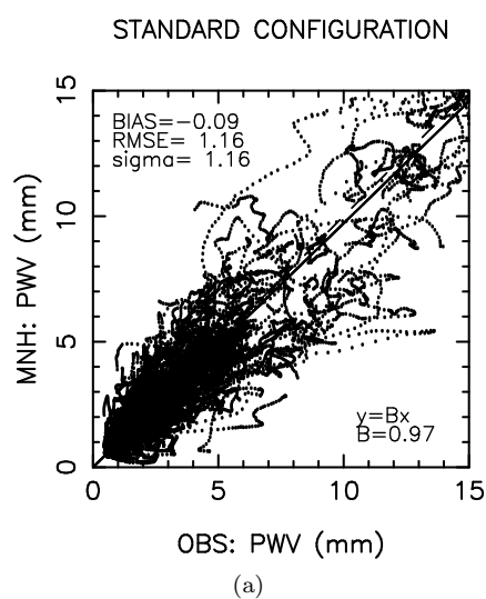
Figure 31: day3 - precipitable water vapor (mm): STANDARD CONFIGURATION
