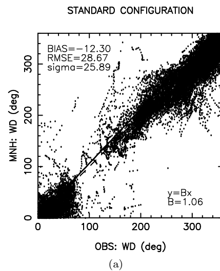
Figure 18: day2 - wind direction (degree): STANDARD CONFIGURATION
