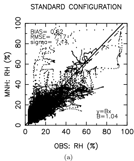
Figure 19: day2 - relative humidity (percent): STANDARD CONFIGURATION
