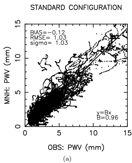
Figure 13: night2 - precipitable water vapor (mm): STANDARD CONFIGURATION
