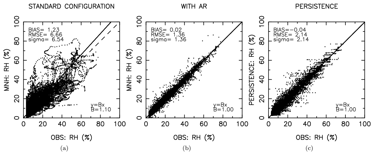
Figure 2: night1 - relative humidity (percent): (a) STANDARD CONFIGURATION, (b) WITH AR (1H), (c) PERSISTENCE (1H)
