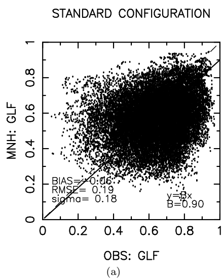
Figure 16: night2 - ground layer fraction (dimensionless): STANDARD CONFIGURATION
