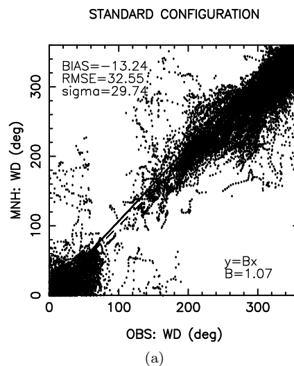
Figure 29: day3 - wind direction (degree): STANDARD CONFIGURATION
