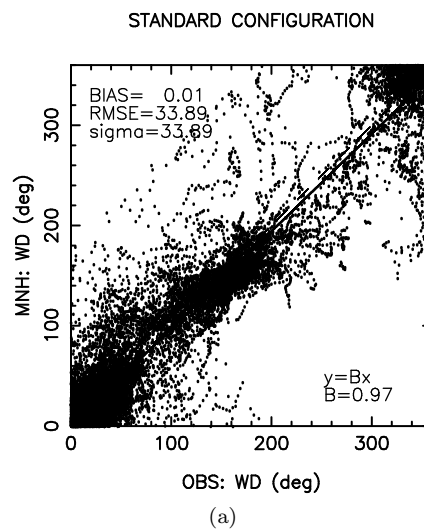
Figure 11: night2 - wind direction (degree): STANDARD CONFIGURATION
