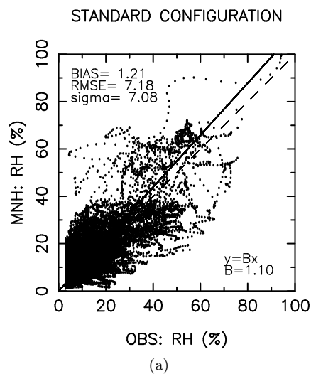
Figure 23: night3 - relative humidity (percent): STANDARD CONFIGURATION
