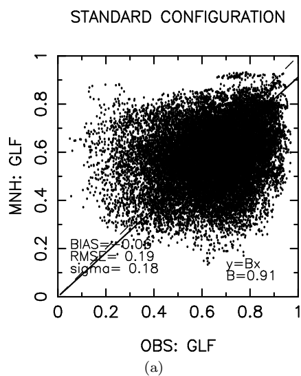
Figure 27: night3 - ground layer fraction (dimensionless): STANDARD CONFIGURATION
