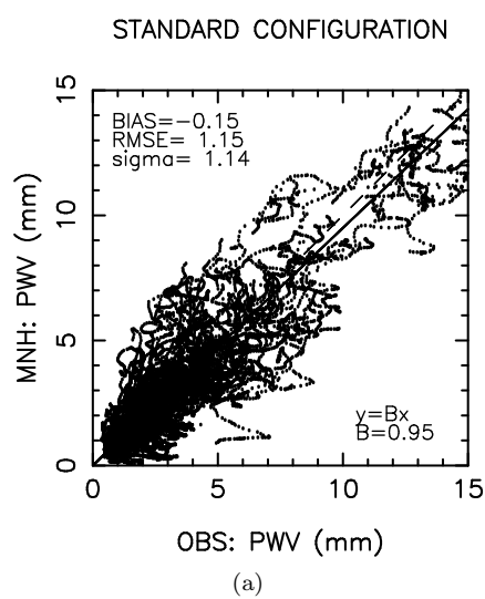
Figure 24: night3 - precipitable water vapor (mm): STANDARD CONFIGURATION
