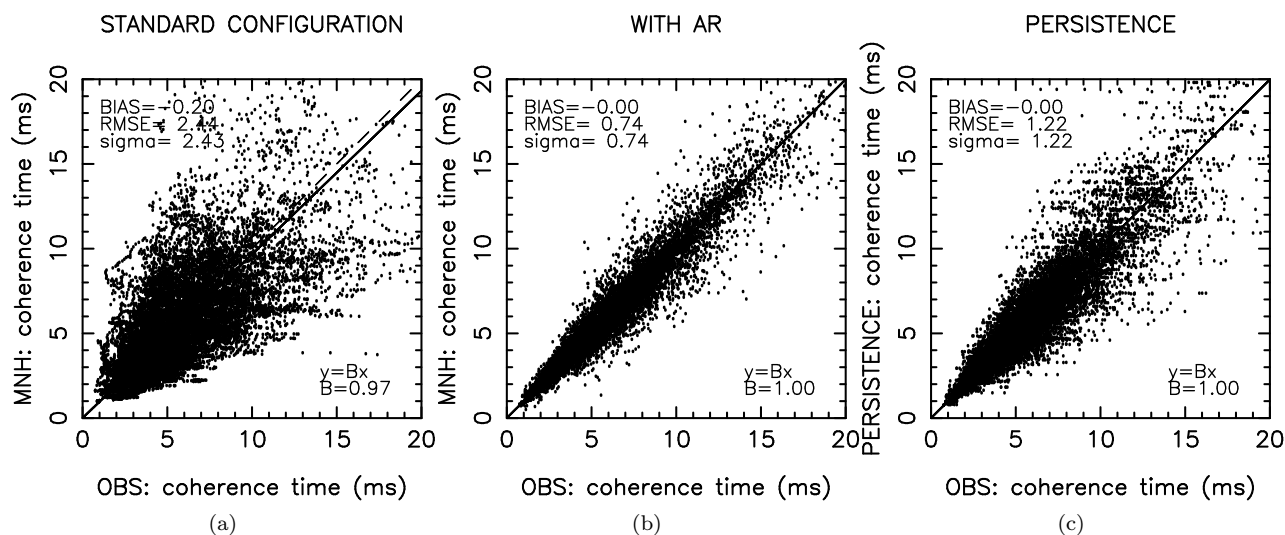
Figure 5: night1 - wavefront coherence time (ms): (a) STANDARD CONFIGURATION, (b) WITH AR (1H), (c) PERSISTENCE (1H)
