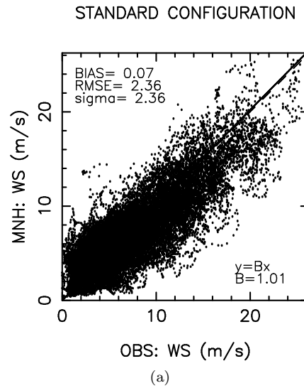
Figure 17: day2 - wind speed ( ms^{-1} ): STANDARD CONFIGURATION
