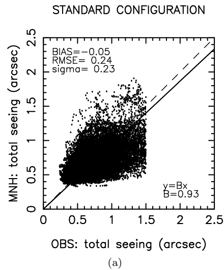
Figure 14: night2 - total seeing (arcsec): STANDARD CONFIGURATION (&lt; 1.5")
