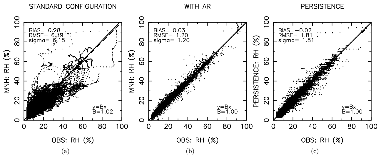
Figure 8: day1 - relative humidity (percent): (a) STANDARD CONFIGURATION, (b) WITH AR (1H), (c) PERSISTENCE (1H)
