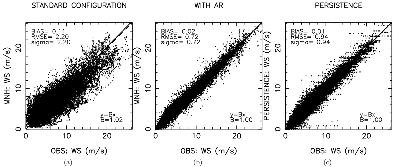
Figure 7: day1 - wind speed ( ms^{-1} ): (a) STANDARD CONFIGURATION, (b) WITH AR (1H), (c) PERSISTENCE (1H)
