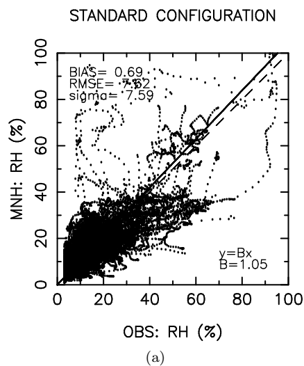
Figure 30: day3 - relative humidity (percent): STANDARD CONFIGURATION
