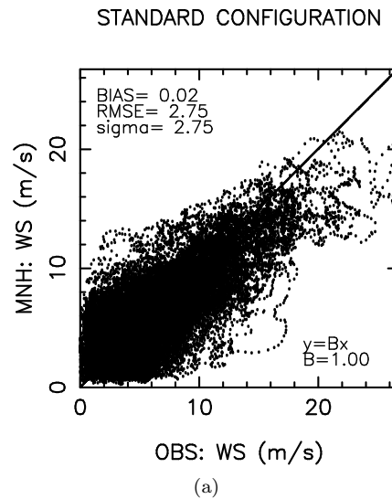
Figure 21: night3 - wind speed ( ms^{-1} ): STANDARD CONFIGURATION
