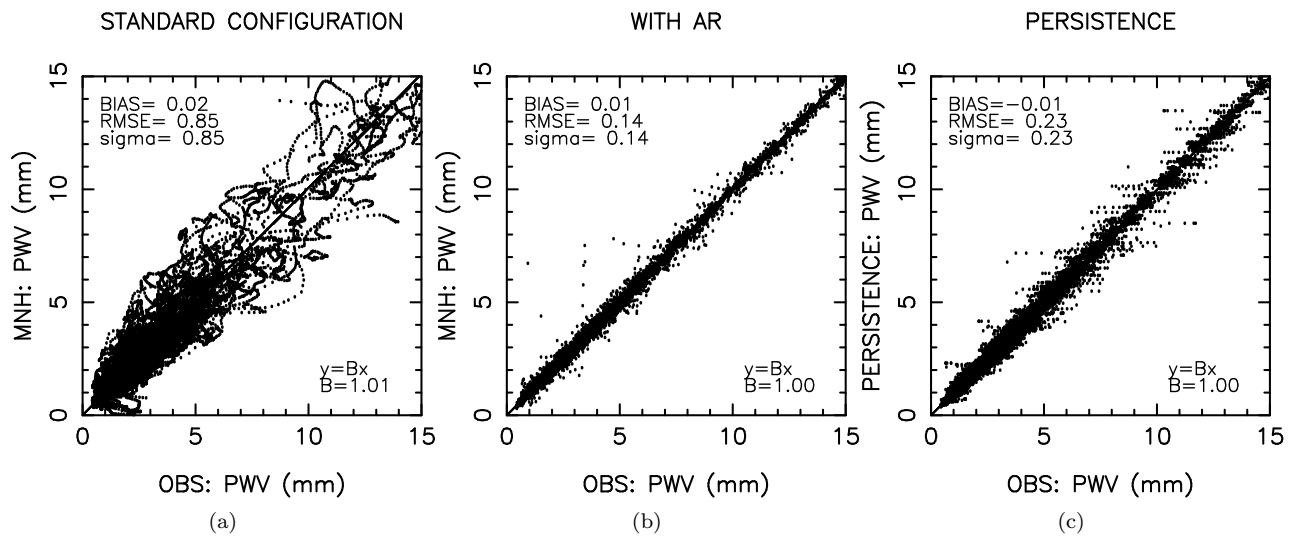
Figure 9: day1 - precipitable water vapor (mm): (a) STANDARD CONFIGURATION, (b) WITH AR (1H), (c) PERSISTENCE (1H)
