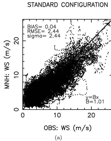
Figure 28: day3 - wind speed ( ms^{-1} ): STANDARD CONFIGURATION
