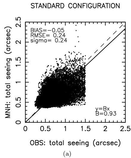
Figure 25: night3 - total seeing (arcsec): STANDARD CONFIGURATION (&lt; 1.5")
