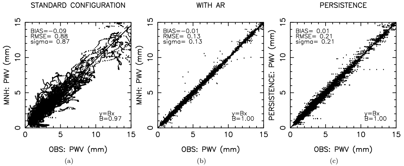
Figure 3: night1 - precipitable water vapor (mm): (a) STANDARD CONFIGURATION, (b) WITH AR (1H), (c) PERSISTENCE (1H)
