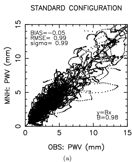
Figure 20: day2 - precipitable water vapor (mm): STANDARD CONFIGURATION
