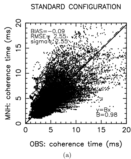
Figure 26: night3 - wavefront coherence time (ms): STANDARD CONFIGURATION
