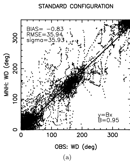
Figure 13: night2 - wind direction (degree): STANDARD CONFIGURATION
