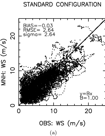
Figure 23: night3 - wind speed ( ms^{-1} ): STANDARD CONFIGURATION
