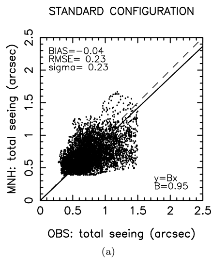
Figure 27: night3 - total seeing (arcsec): STANDARD CONFIGURATION (< 1.5")
