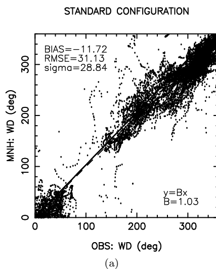
Figure 31: day3 - wind direction (degree): STANDARD CONFIGURATION
