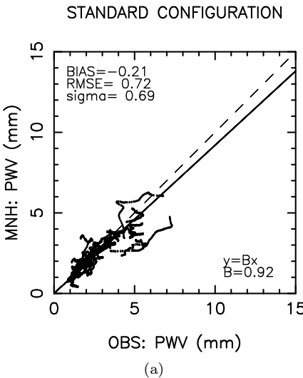
Figure 22: day2 - precipitable water vapor (mm): STANDARD CONFIGURATION
