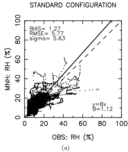
Figure 32: day3 - relative humidity (percent): STANDARD CONFIGURATION
