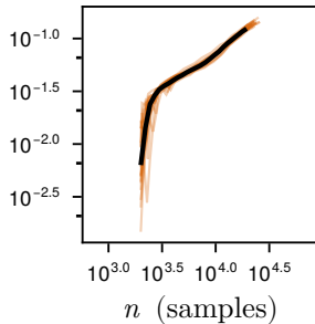
MoleWhacker
