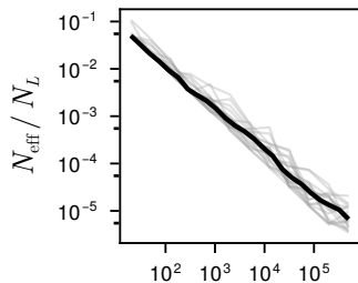
IS
