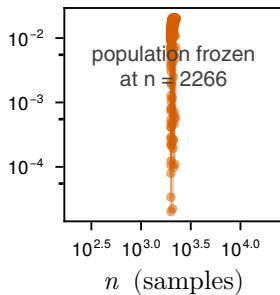
MoleWhacker
