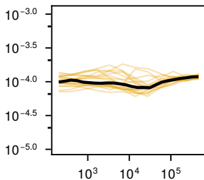
MH
