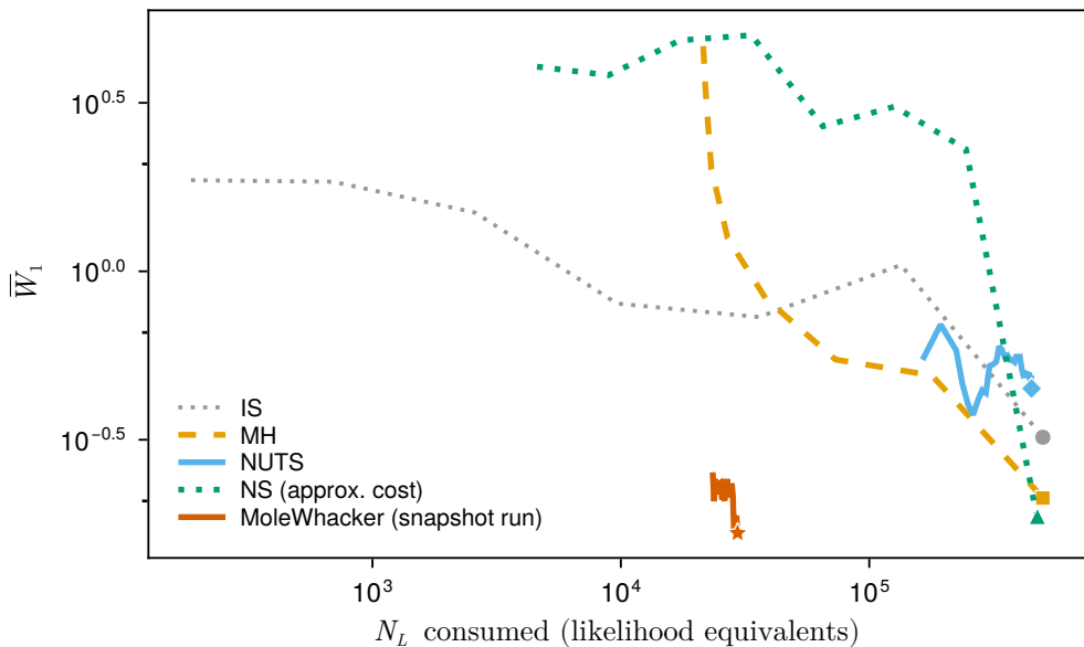
M-Ridges, d = 5 , B = 5 \times 10^5
