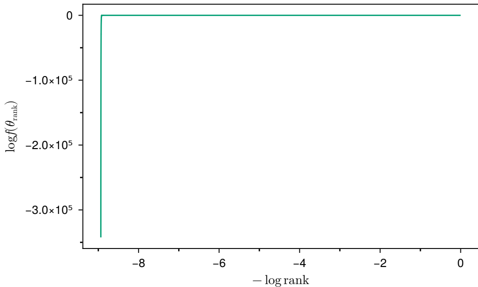
NS posterior log — density across draws (sorted)
