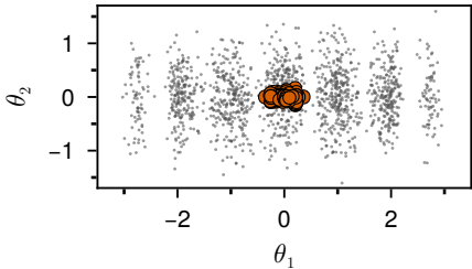
MW component centres
