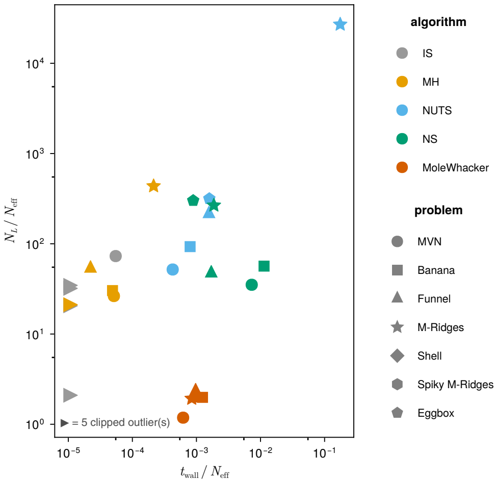
Cross-problem Pareto ( d = 2 , B = 5 \times 10^5 )
