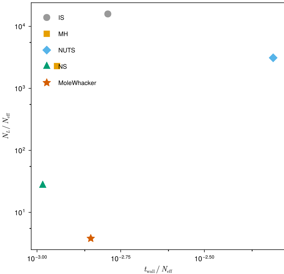
Funnel ( d = 5 , B = 5 \times 10^5 )
