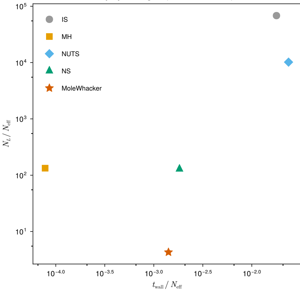
Spiky M-Ridges ( d = 5 , B = 5 \times 10^5 )
