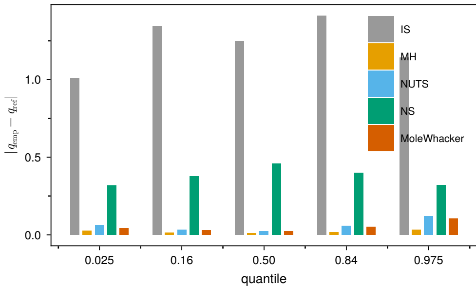
Banana ( d = 10 , B = 5 \times 10^5 )
