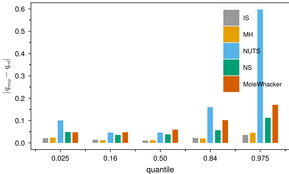
Banana ( d = 2 , B = 5 \times 10^5 )
