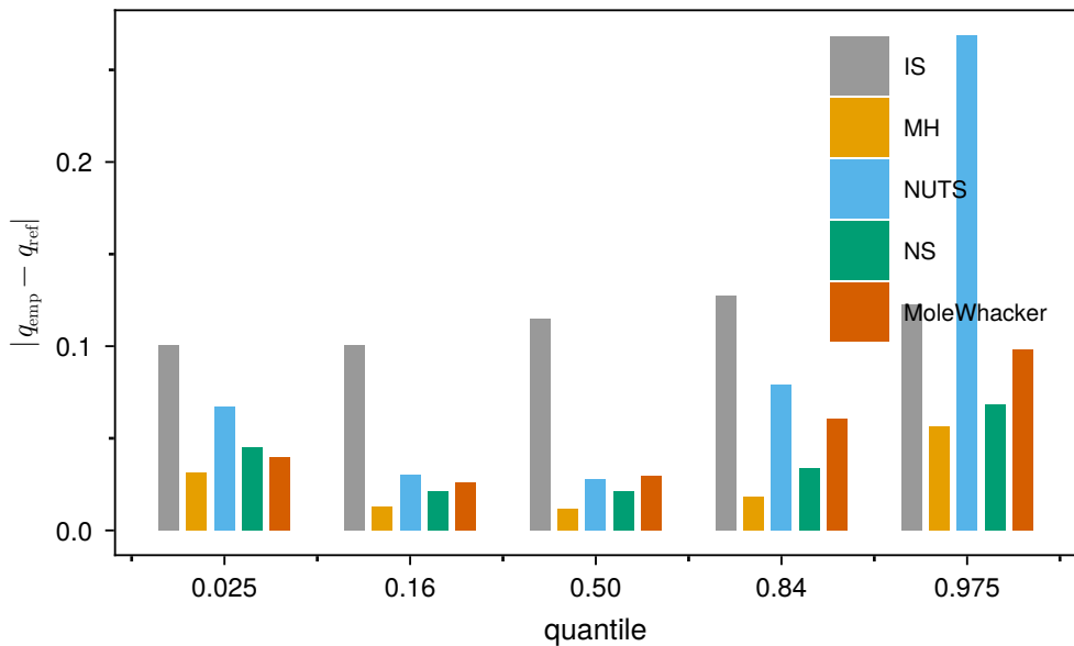
Banana ( d = 5 , B = 5 \times 10^5 )
