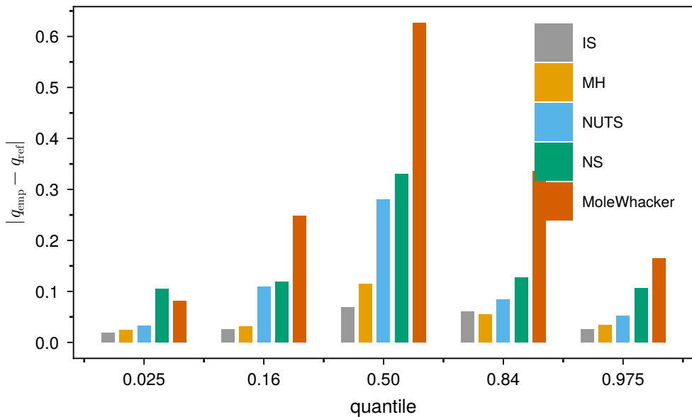
Eggbox ( d = 2 , B = 5 \times 10^5 )
