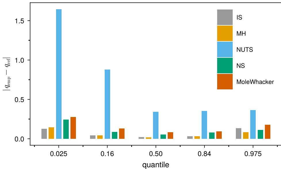
Funnel ( d = 2 , B = 5 \times 10^5 )
