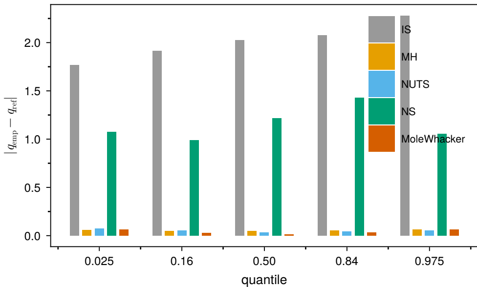
MVN ( d = 10 , B = 5 \times 10^5 )
