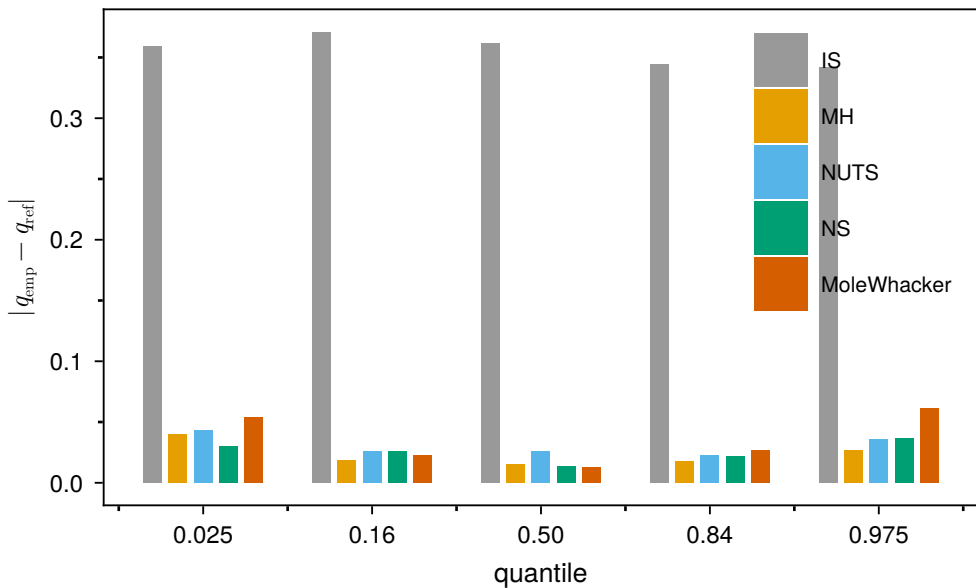
MVN ( d = 5 , B = 5 \times 10^5 )
