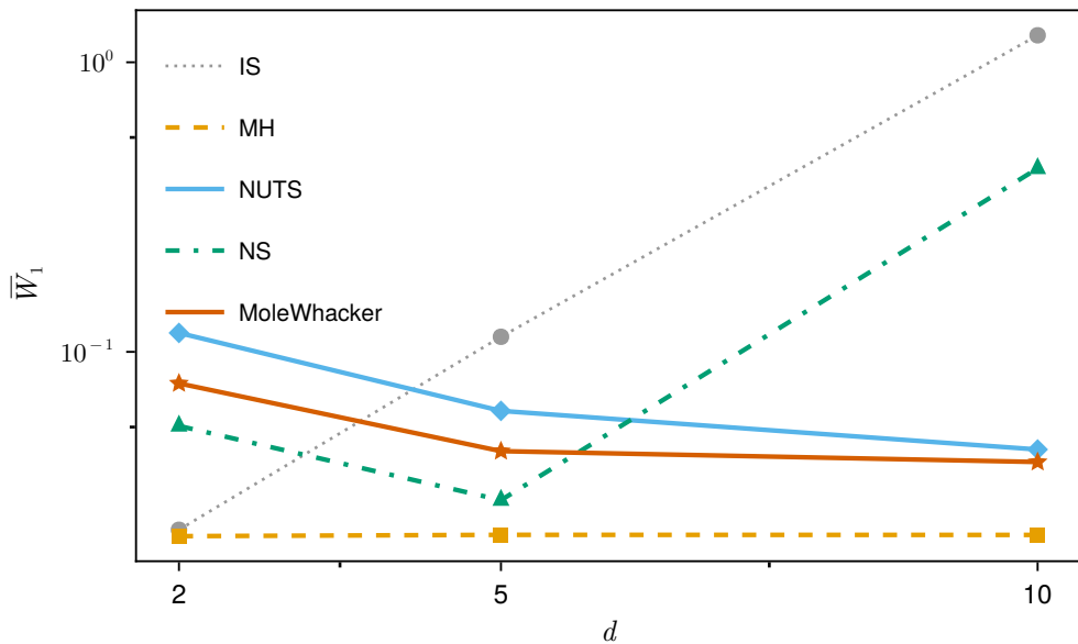
Banana, scaling at B = 5 \times 10^5
