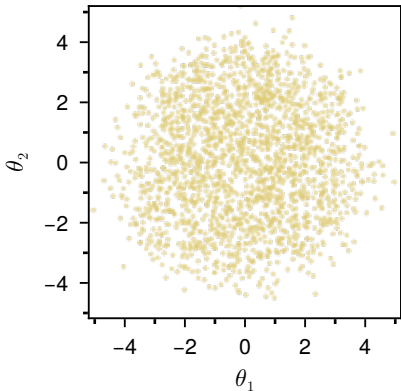
Shell, truth samples
