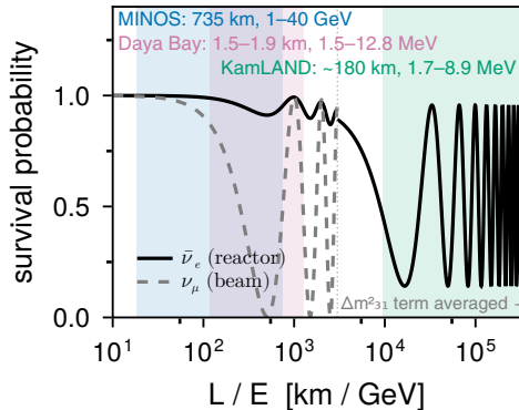
(a) three-flavor vacuum oscillations
