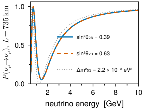
(b) the \theta_{23} octant degeneracy
