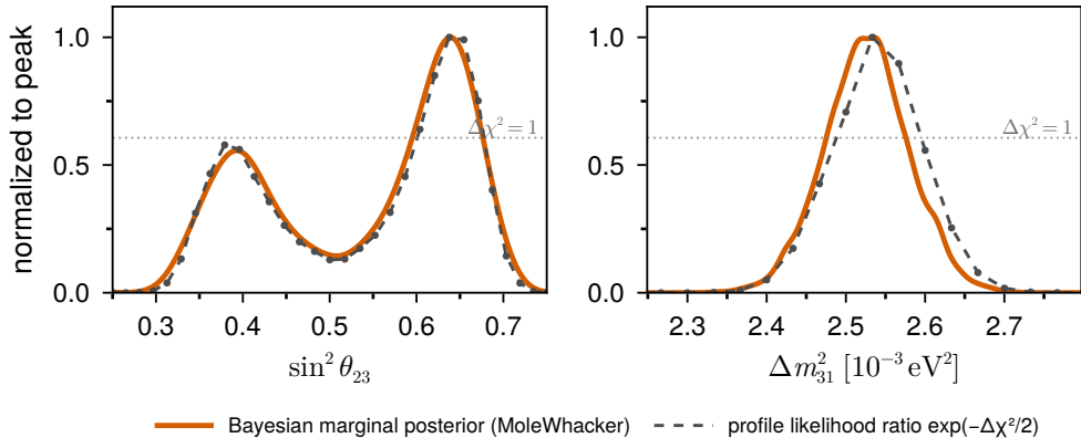
Normal ordering: Bayesian marginal vs. profile likelihood
