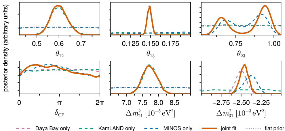
Inverted ordering: single-experiment fits ( B = 5 \times 10^4 ) and the joint fit ( B = 5 \times 10^5 )
