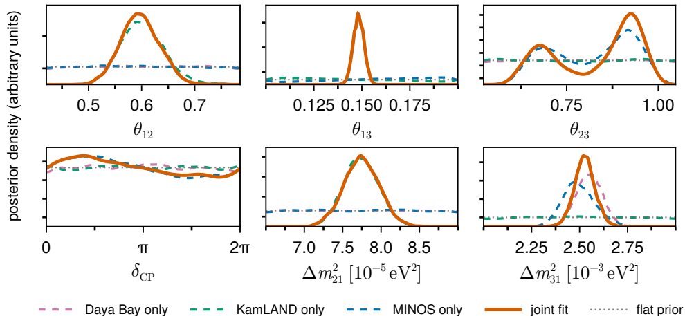
Normal ordering: single-experiment fits ( B = 5 \times 10^4 ) and the joint fit ( B = 5 \times 10^5 )
