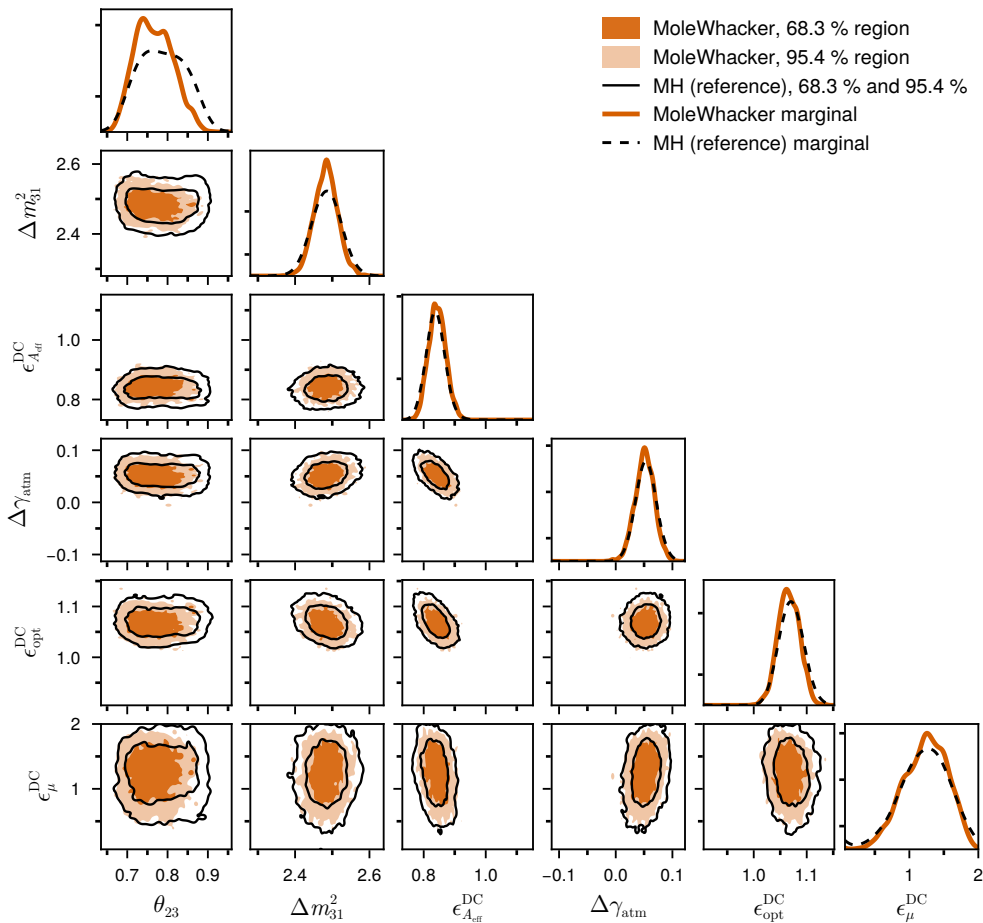
Four experiments, normal ordering, B = 5 \times 10^5 : atmospheric sector and correlated DeepCore nuisance parameter ( \theta_{23} in rad, \Delta m_{31}^2 in 10^{-3} \text{ eV}^2 ; 3 \times 10^4 draws per sampler, seeds pooled)
