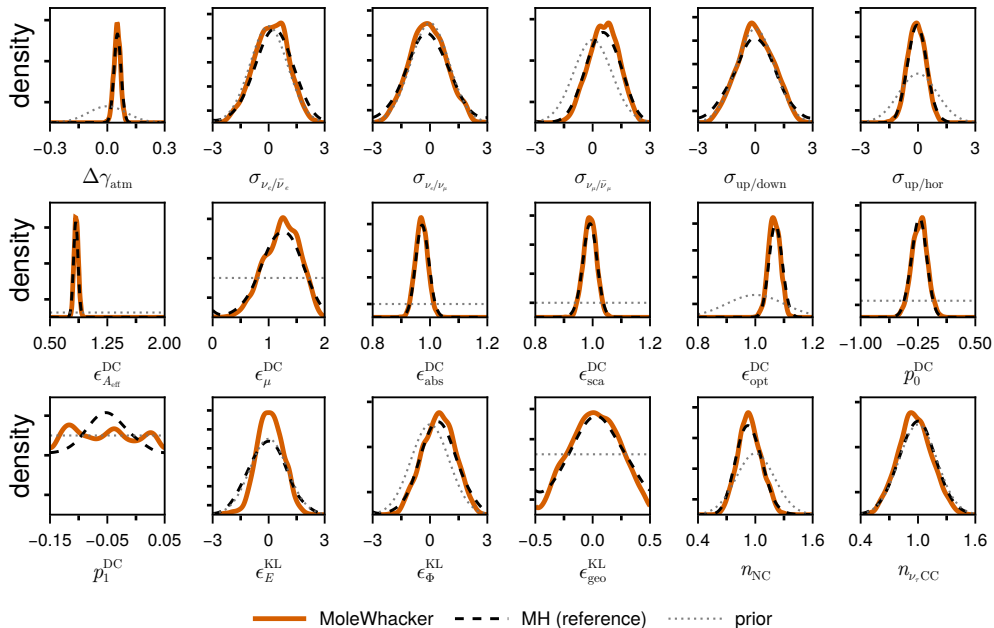
Nuisance parameters of the four-experiment fit, normal ordering, B = 5 \times 10^5
