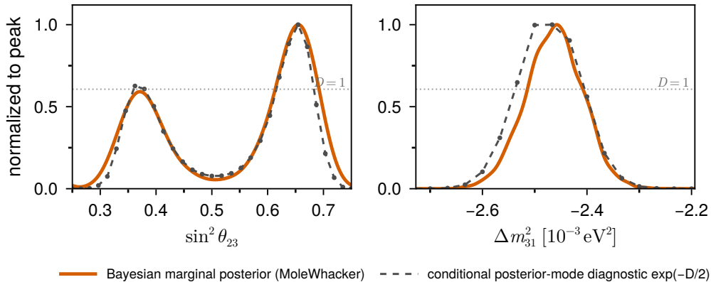
Inverted ordering: Bayesian marginal vs. conditional posterior-mode diagnostic
