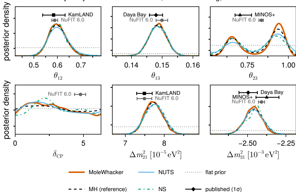
Daya Bay + KamLAND + MINOS, inverted ordering, B = 5 \times 10^5
