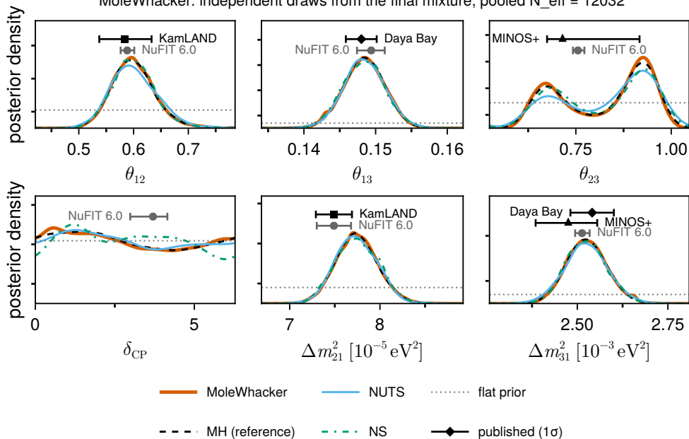
Daya Bay + KamLAND + MINOS, normal ordering, B = 5 \times 10^5 MoleWhacker: independent draws from the final mixture, pooled N_{\text{eff}} = 12032
