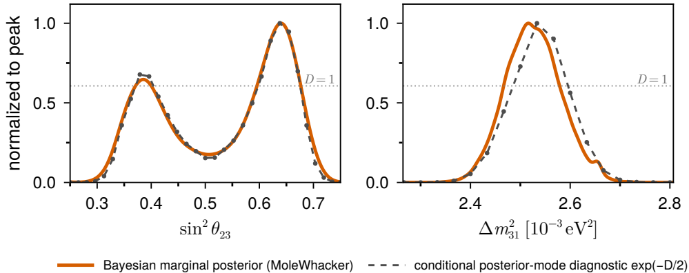
Normal ordering: Bayesian marginal vs. conditional posterior-mode diagnostic
