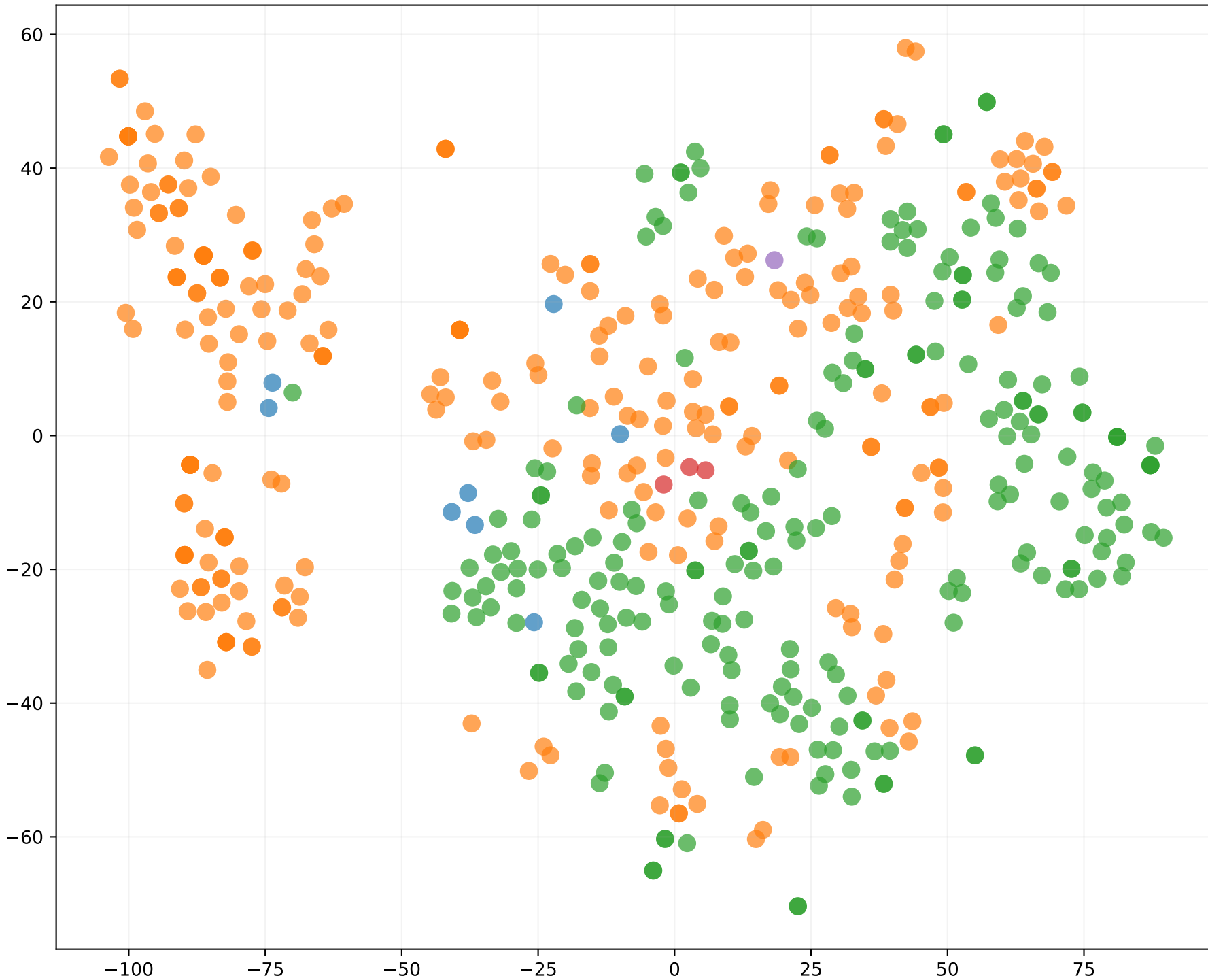
W2V Context Space: 'mw' (Avg Context, window=3)
