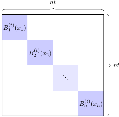
Fig. 5: Construction of B^{(t)}(x) from the B_i^{(t)}(x_i) for i \in [n] .
