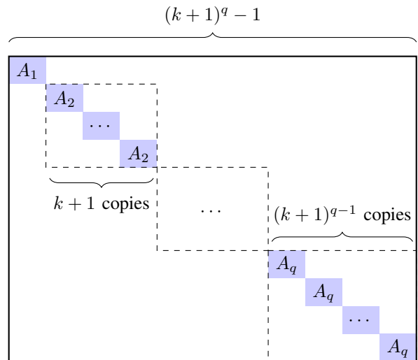
Fig. 4: Construction of the matrix A(x) from the matrices A_i(x_i) with i \in [q] .
