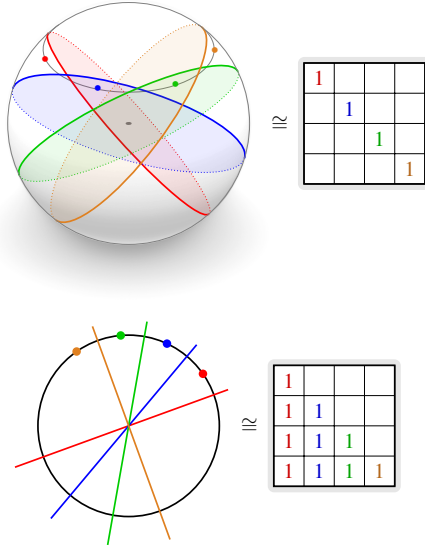
Fig. 1: Sign-rank representations of the identity matrix and lower triangular matrix.
