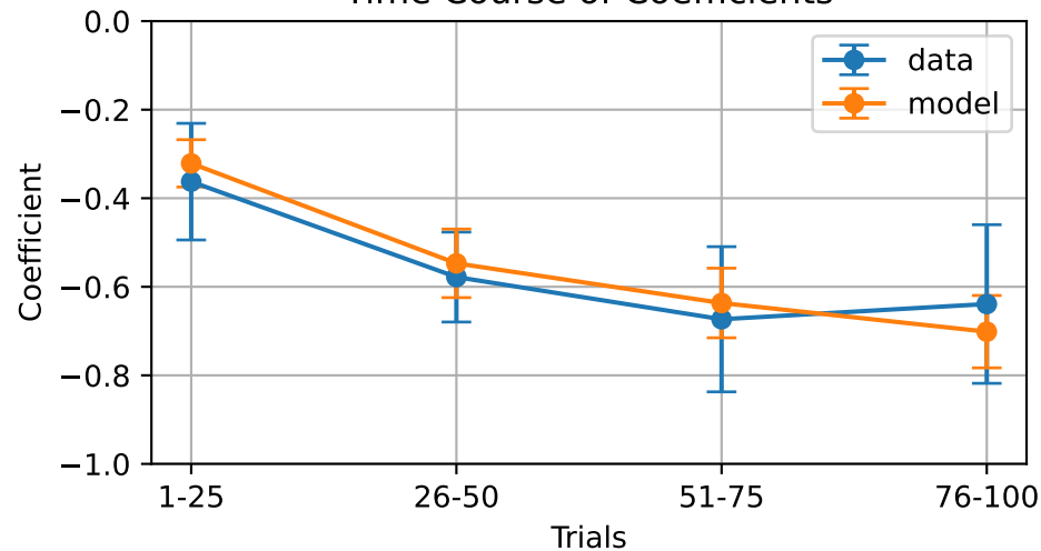
Time Course of Coefficients
