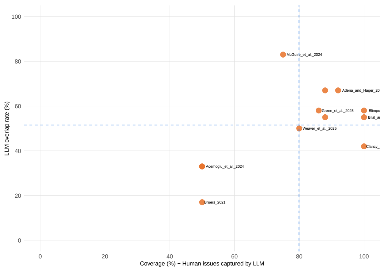
Figure 3: Coverage (% of human-identified issues that the LLM also raised) vs LLM overlap rate (% of LLM-raised issues that match a substantive human concern) for each paper, as assessed by GPT-5.2 Pro acting as judge. Dashed lines mark the cross-paper mean for each axis. Papers in the upper-right quadrant show strong alignment between human and LLM critiques.
