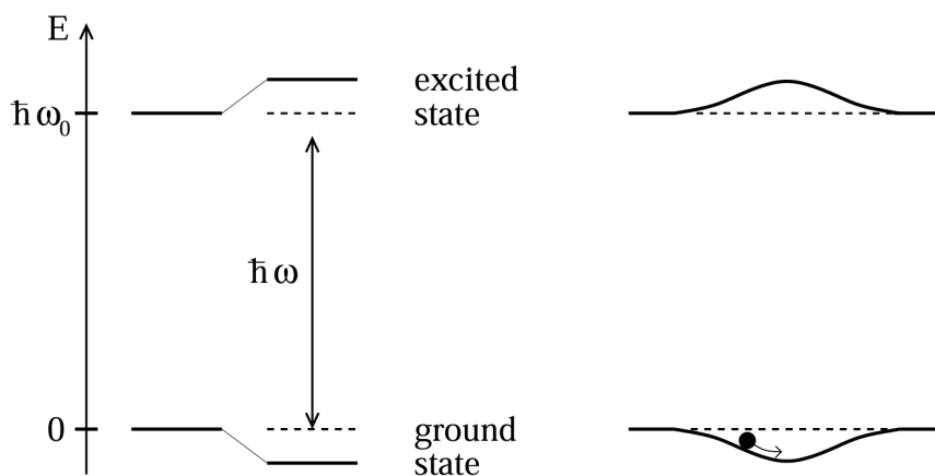
Figure 1.7: Light shifts for a two-level atom. Left: red-detuned light ( \Delta < 0 ) shifts the ground state down and the excited state up by equal amounts. Right: a spatially inhomogeneous field such as a Gaussian laser beam produces a ground-state potential well in which an atom can be trapped.
