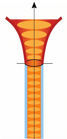
Figure 1.9: The strongly anisotropic, disc-shaped potential wells of the one-dimensional optical lattice.
