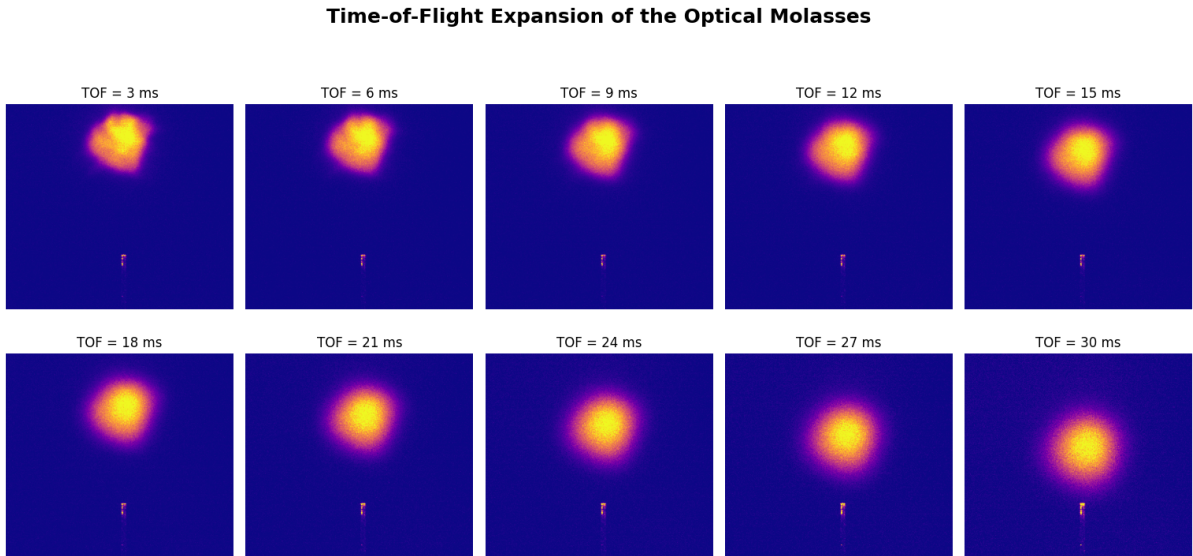
Figure 1.1: Fluorescence images of the atomic cloud recorded during Time-of-Flight expansion, with expansion times ranging from 3.0 ms to 30.0 ms.
