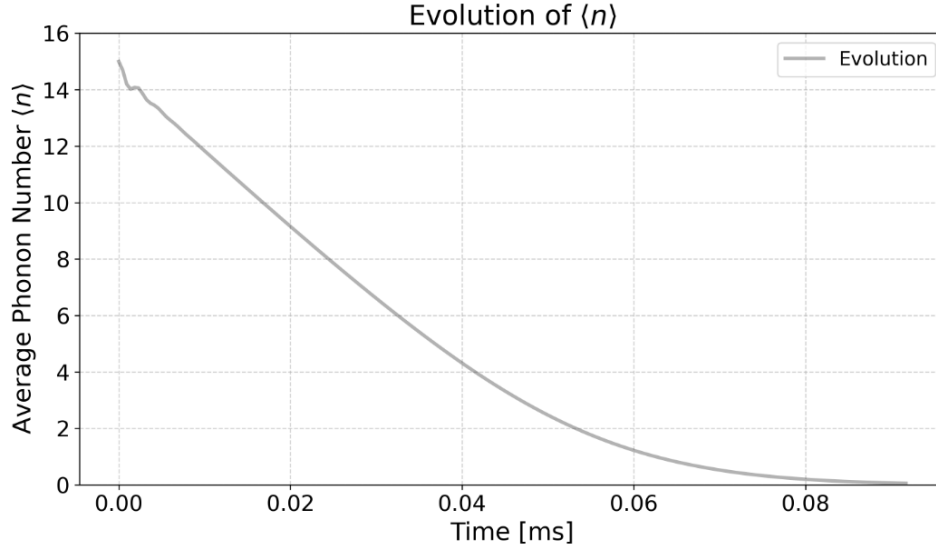
Figure 1.16: Time evolution of the average phonon number \langle n \rangle in the three-level simulation. The population rapidly cools to the motional ground state within approximately 0.1 ms.
